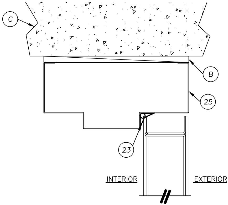
1 VERTICAL CROSS SECTION 6 @ HEAD
