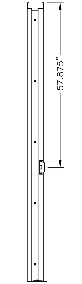
STRIKE PLATE LOCATION 2" HEAD
