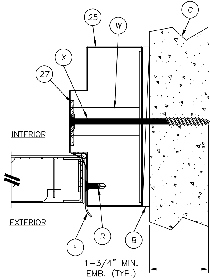
2 3 HORIZONTAL CROSS SECTION @ LATCH SHOWN WITH TUBE ANCHOR
