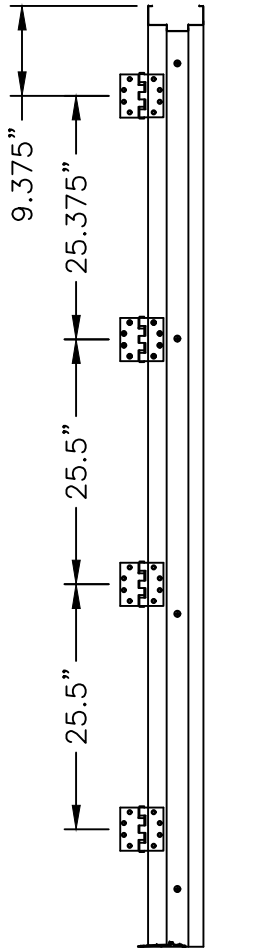
HINGE LOCATIONS 2" HEAD
